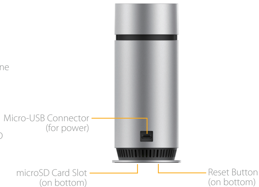
Back View
